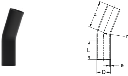
BR PE100 Rohrbogen 22° nahtlos lang SDR11 schwarz BR PE100 Pipe bend 22° seamless long SDR11 black
