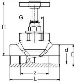
BR PP-RCT-Ms Ventil Geradsitz Handrad grün BR PP-RCT-Brass Valve straight with hand wheel green
