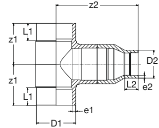
BR PP-RCT T-Stück 90° red Form-B lang st grün BR PP-RCT Tee 90° red style-B long butt green
