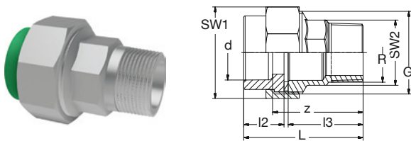
BR PP-RCT-V2A Ü-Verschraubung AG-keg Flachdichtring-EPDM 20°C/1.0MPa grün BR PP-RCT- Stainless steel Transition-Union male-thread-con flat-gasket-EPDM 20°C/1.0MPa green
