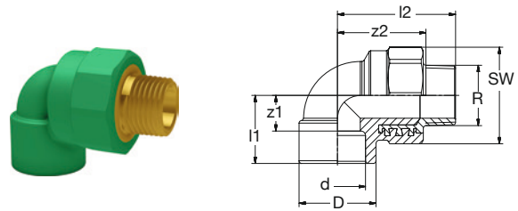
BR PP-RCT-LFB Ü-Winkel 90° AG-keg grün BR PP-RCT-LFB Transition-Elbow 90° male-thread-con green
