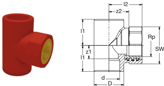
BR PP-CFR- LFB Ü-T-Stück 90° IG-zyl rot
