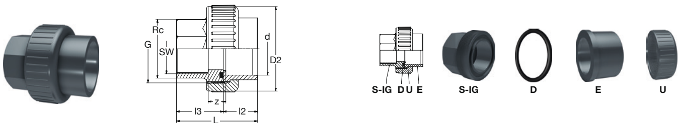
BR PVC-U Ü-Verschraubung IG-keg Runddichtring-EPDM grau BR PVC-U Transition-Union female-thread-con O-Ring-gasket-EPDM grey
