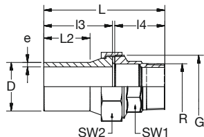
BR PE100- V2A Ü-Verschraubung lang AG-keg Flachdichtring-EPDM SDR11 schwarz BR PE100- Stainless steel Transition-Union long male-thread-con flat-gasket-EPDM SDR11 black
