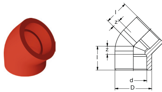
BR PP-CFR Winkel 45° rot
