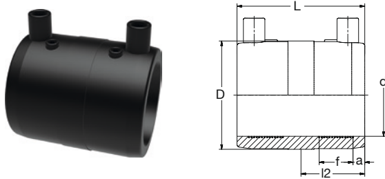
BR PE100 E-Muffe SDR11 schwarz
