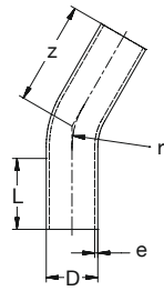
BR PE100 Rohrbogen 30° nahtlos lang SDR11 schwarz BR PE100 Pipe bend 30° seamless long SDR11 black
