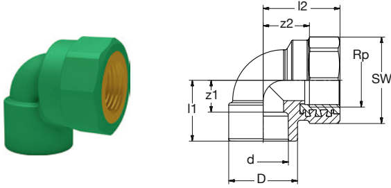
BR PP-RCT-RG/LFB Ü-Winkel 90° IG-zyl grün BR PP-RCT-Bronze/LFB Transition-Elbow 90° female-thread-cyl green
