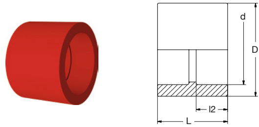
BR PP-CFR Muffe rot BR PP-CFR Socket red
