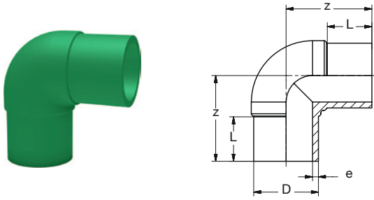
BR PP-RCT Winkel 90° lang st grün BR PP-RCT Elbow 90° long butt green
