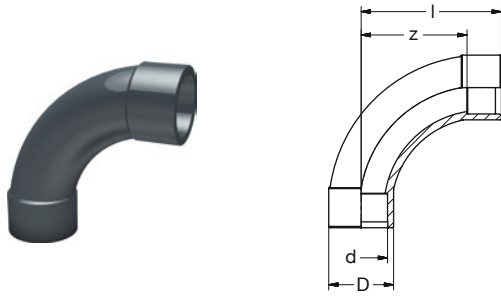
BR PVC-U Bogen 90° grau BR PVC-U Bend 90° grey
