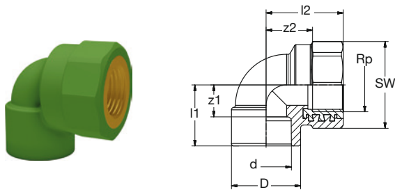
BR PP-R-RG/LFB Ü-Winkel 90° IG-zyl grün
