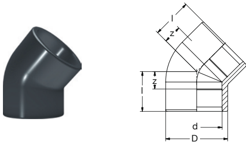
BR PVC-U Winkel 45° grau BR PVC-U Elbow 45° grey
