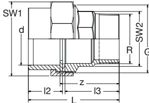
BR PVC-U- V2A Ü-Verschraubung AG-keg Flachdichtring-EPDM grau BR PVC-U- Stainless Steel Transition-Union male-thread-con flat-gasket-EPDM grey
