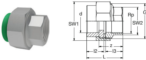
BR PP-RCT-V2A Ü-Verschraubung IG-zyf Flachdichtring-EPDM 20°C/1,0MPa grün BR PP-RCT- Stainless steel Transition-Union female-thread-cyl flat-gasket-EPDM 20°C/1.0MPa green
