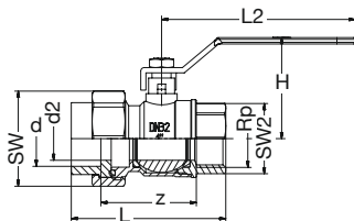
BR PP-RCT Ü-Kugelhahn-Messing IG-zyl verschraubt Runddichtring-EPDM 20°C/1,0MPa grün BR PP-RCT Transition-Ball valve Brass female-thread-cyl with union-nuts O-Ring-gasket-EPDM 20°C/1.0MPa green
