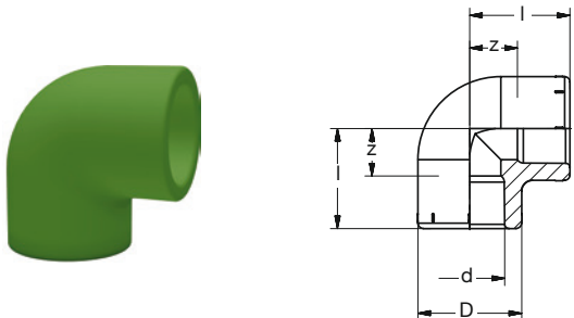
BR PP-R Winkel 90° grün BR PP-R Elbow 90° green
