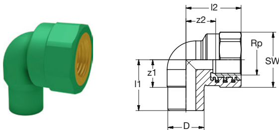
BR PP-RCT-RG/LFB Ü-Winkel 90° i IG-zyl grün BR PP-RCT-Bronze/LFB Transition-Elbow 90° fem female-thread-cyl green
