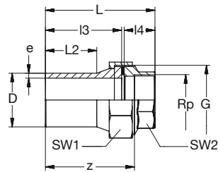
BR PE100- V2A Ü-Verschraubung lang IG-zyf Flachdichtring-EPDM SDR11 schwarz BR PE100- Stainless steel Transition-Union long female-thread-cyl SDR11 black
