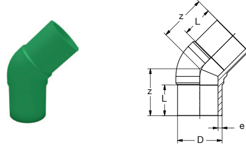
BR PP-RCT Winkel 45° lang st grün BR PP-RCT Elbow 45° long butt green
