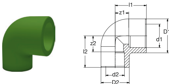
BR PP-R Winkel 90° red grün BR PP-R Elbow 90° red. green
