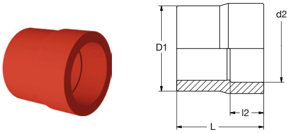
BR PP-CFR Reduktion rot BR PP-CFR Reducer red
