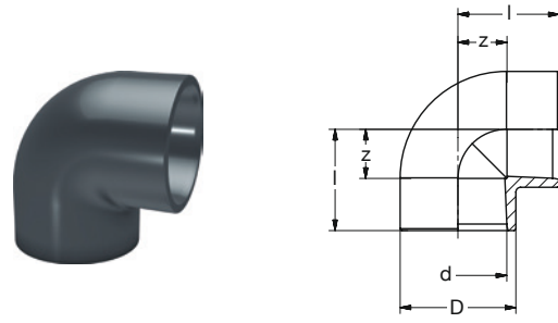
BR PVC-U Winkel 90° grau BR PVC-U Elbow 90° grey
