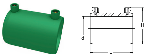
PP-RCT E-Muffe grün PP-RCT E-Socket green
