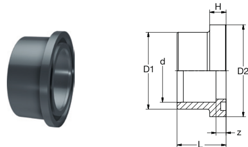
BR PVC-U Bundbuchse O-Ring-Kammer grau BR PVC-U Flange adaptor socket O-Ring-chamber grey
