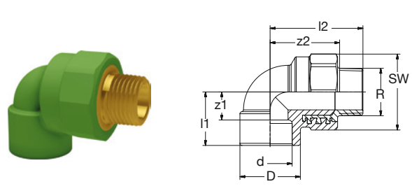
BR PP-R-RG/LFB Ü-Winkel 90° AG-keg grün
