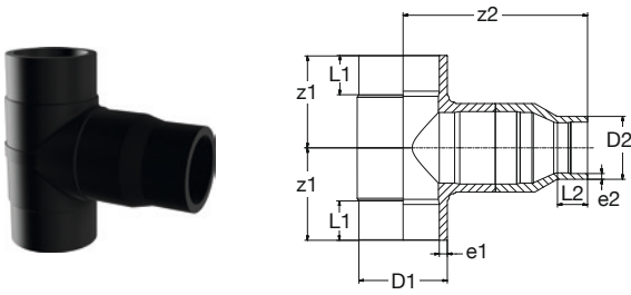
BR PE100 T-Stück 90° red lang Form-B SDR11 schwarz BR PE100 Tee 90° red long style-B SDR11 black
