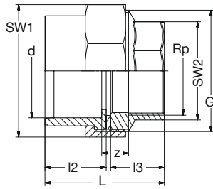
BR PVC-U- V2A Ü-Verschraubung IG-zyl Flachdichtring-EPDM grau BR PVC-U- Stainless Steel Transition-Union female-thread-cyl flat-gasket-EPDM grey
