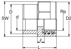
BR PVC-U-RG/LFB Übergang IG-zyl grau BR PVC-U-Bronze/LFB Transition female-thread-cyl grey
